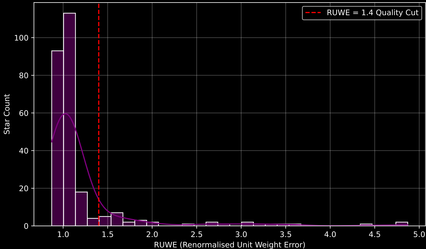
GALAH DR4 Field [2057] RUWE Distribution (n= 260)
