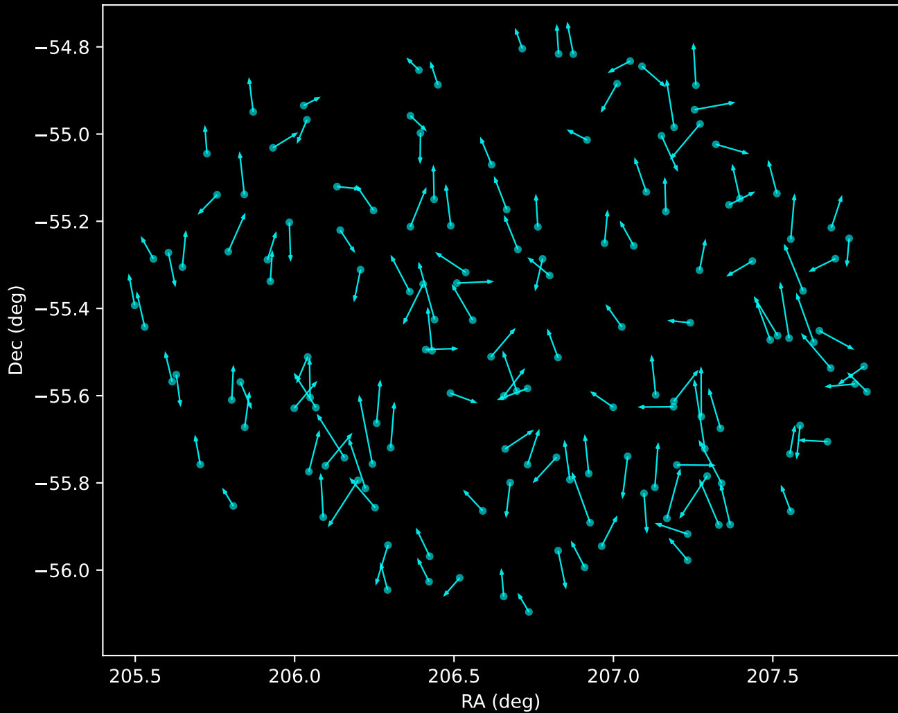
GALAH DR4 Noise Stream Proper Motion Vectors (n=146)
