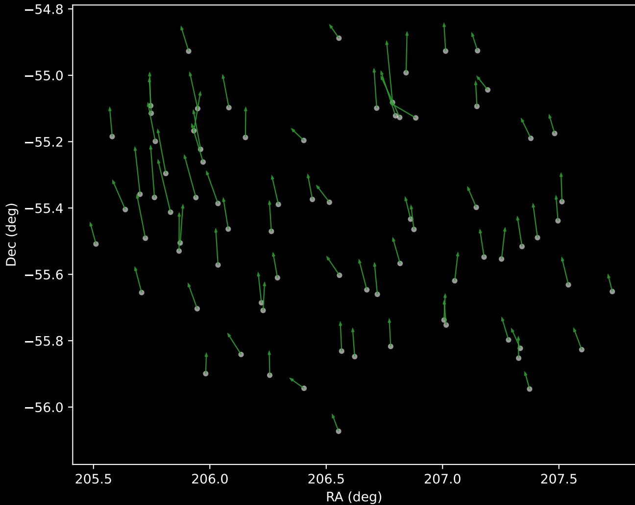
GALAH DR4 Cluster 4 Proper Motion Vectors (n=78)
